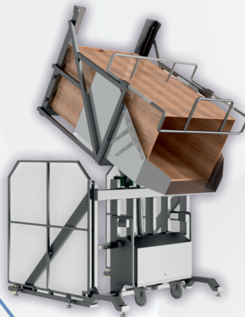
SPECIAL TIPPERS
